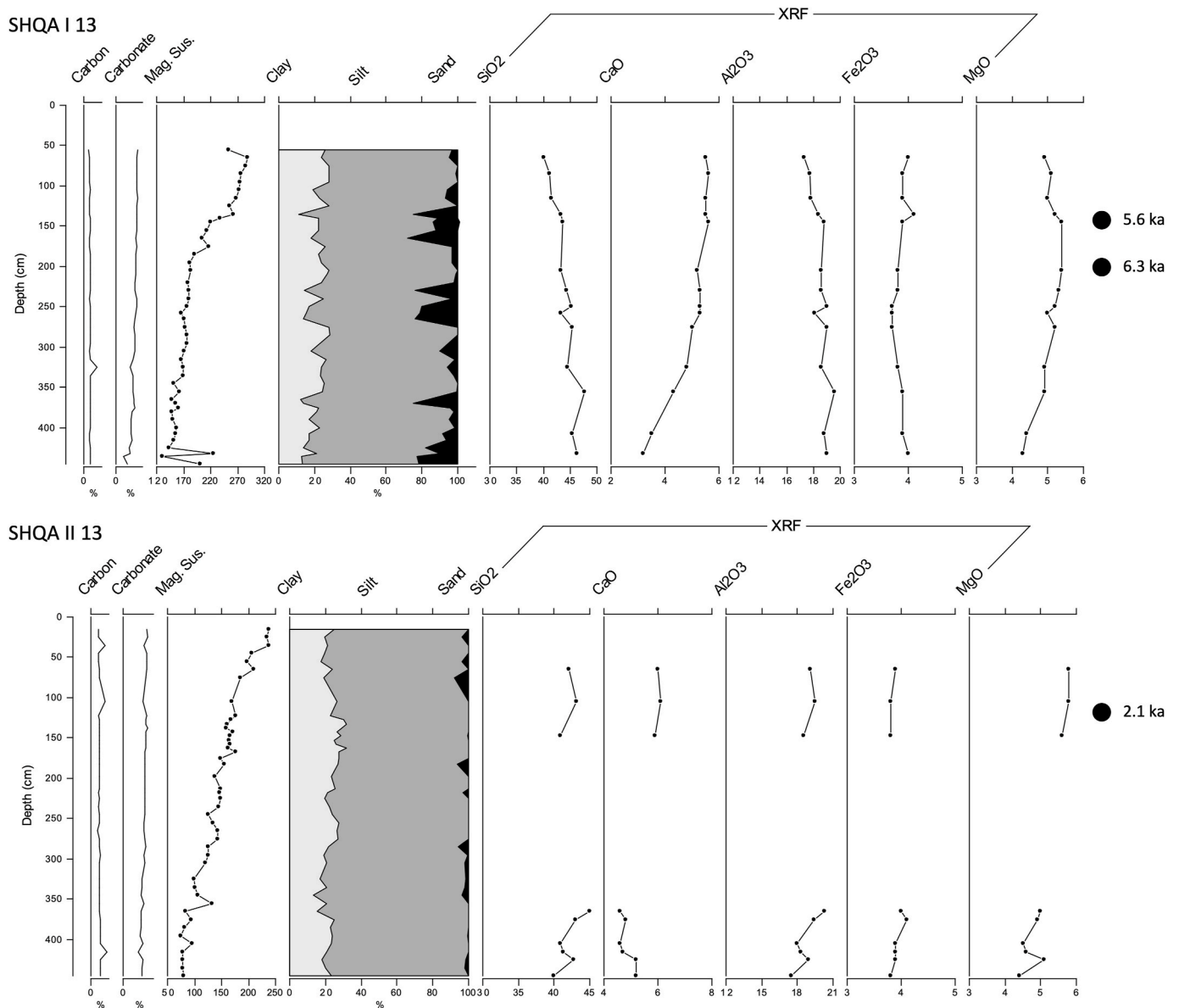
Fig. 4. Sediment analyses from Qa' Shubayqa, showing changes through two sections section from the site. Estimates of percentage carbon and carbonate from LOI, magnetic susceptibility, percentage of clays, silts and sands from the grain size analyses and key elemental compositions from XRF.
