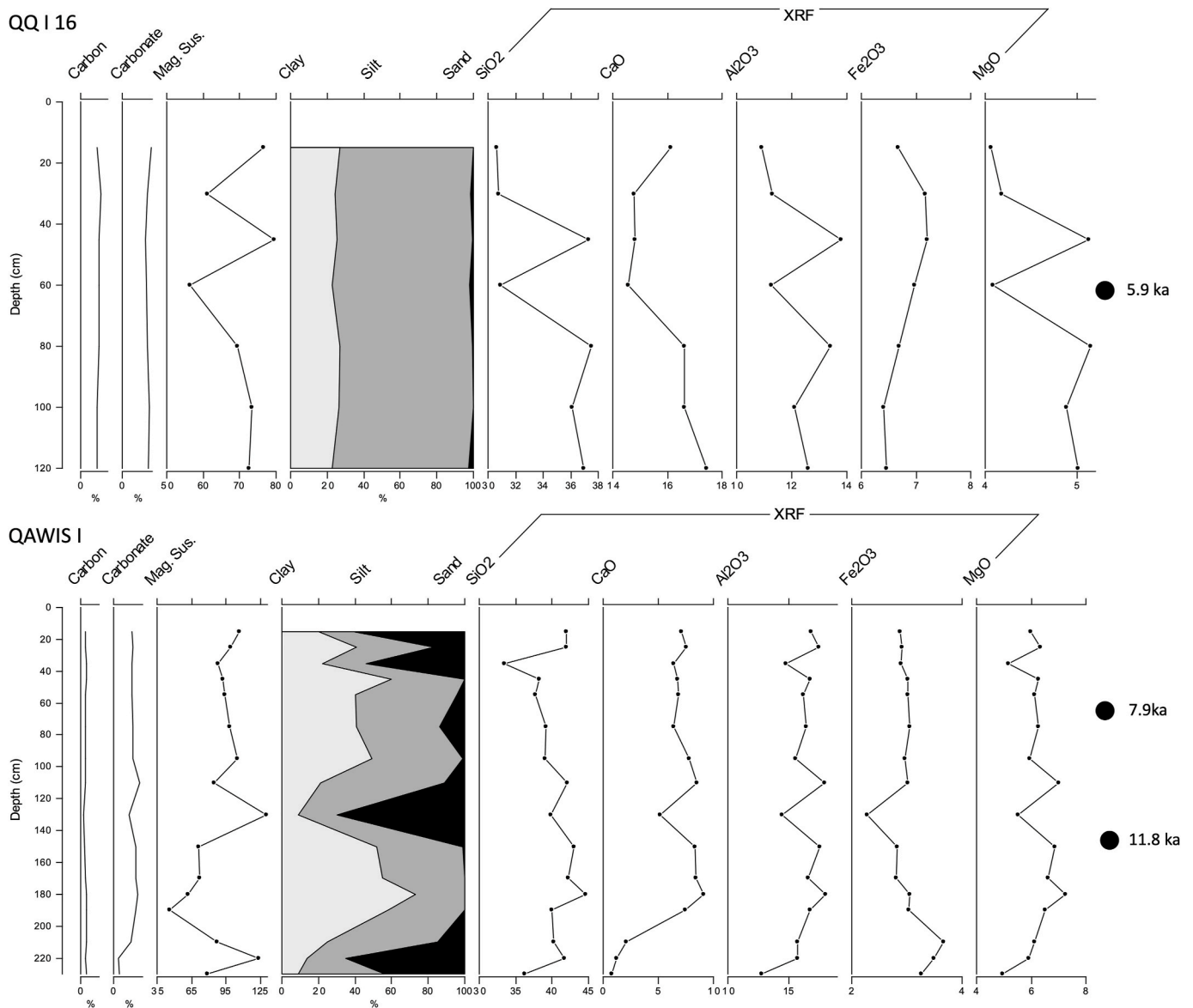
Fig. 3. Sediment analyses from Qa' Qattafi and Qa' Wisad, showing changes through an example section from each site. Estimates of percentage carbon and carbonate from LOI, magnetic susceptibility, percentage of clays, silts and sands from the grain size analyses and key elemental compositions from XRF.
