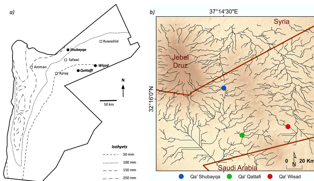
Fig. 1. a) Map of Jordan showing the study sites (and selected present day occupation centres) with the rainfall isolines b) primary wadi drainage in the eastern Jordanian Badia. The drainage network was produced using the SRTM v3 (30 m pixel) Digital Elevation Model (DEM) and the Hydrology Toolset in ArcMap v.10.3.1.
