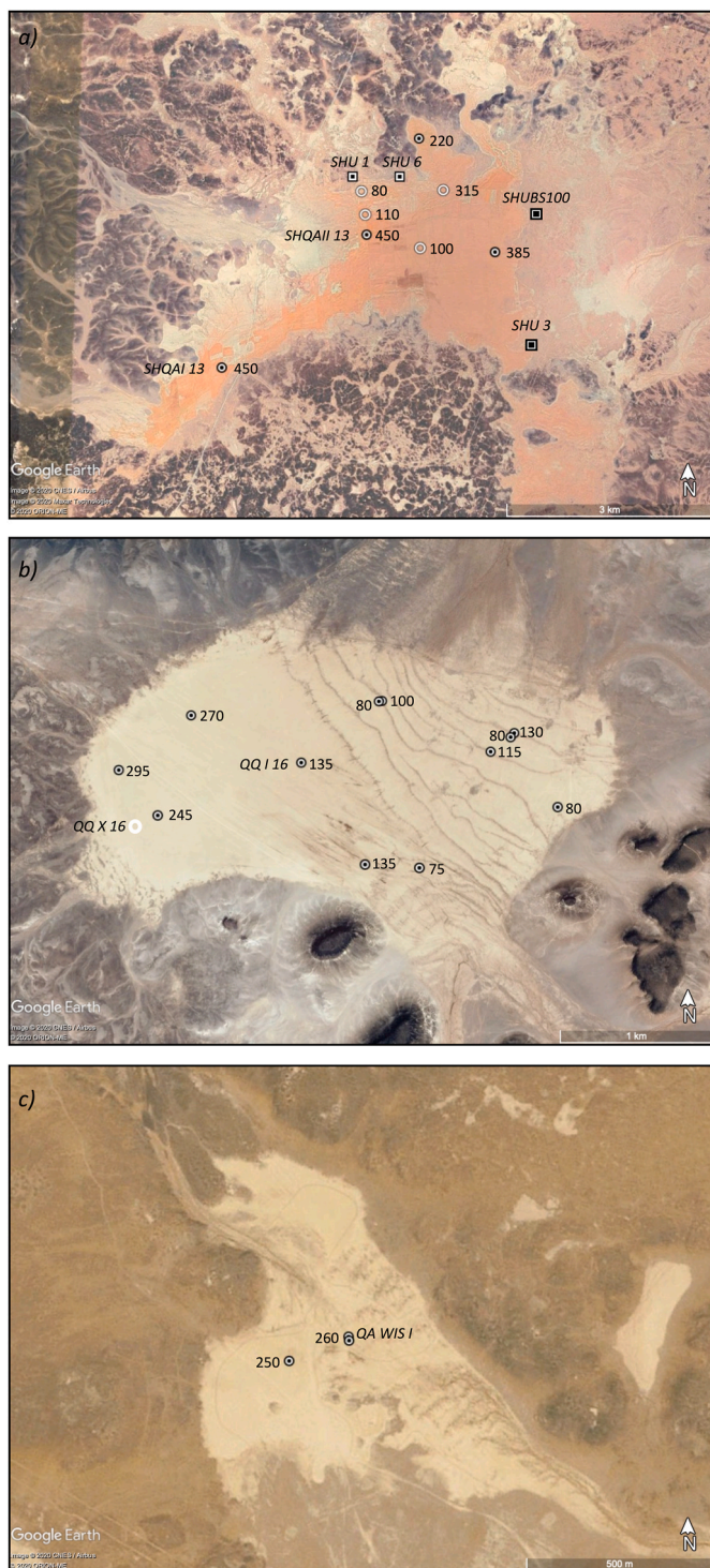
Fig. 2. The three sites Qa' Shubayqa (a), Qa' Qattafi (b) and Qa' Wisad (c) showing measured sediment depths (m), sampled sections referred to in the text are named. Key archaeological sites around Qa' Shubayqa (a) are marked (squares) and open circles mark partial sediment depths for this site.
